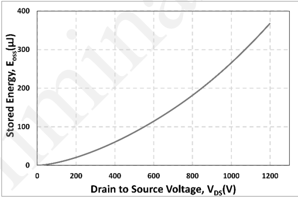
Figure 10. Output Capacitor Stored Energy
