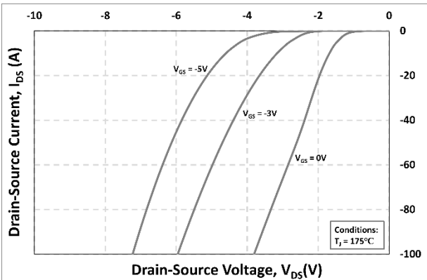
Figure 6. Body Diode Characteristic at 175^\circ\text{C}
