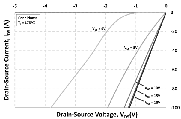
Figure 12. 3rd Quadrant Characteristic at 175°C
