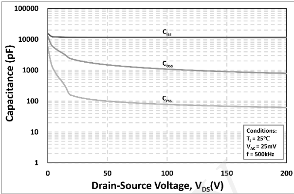
Figure 8. Capacitances vs. Drain-Source Voltage (0 - 200V)
