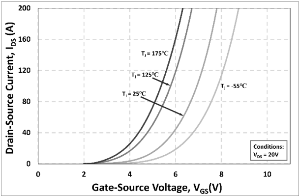
Figure 13. Transfer Characteristic for Various Junction Temperatures
