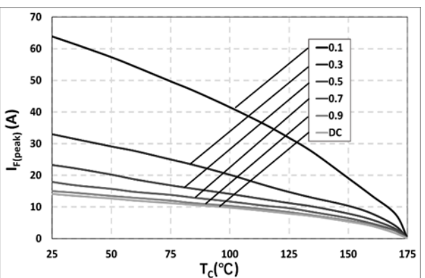
Fig. 6 Current Derating
